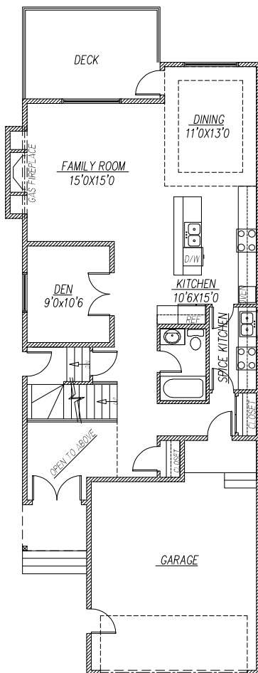
MAIN FLOOR PLAN (WITH SPICE KITCHEN) 1127 SQ FT
