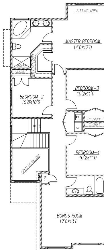
UPPER FLOOR PLAN 1343 SQ FT
